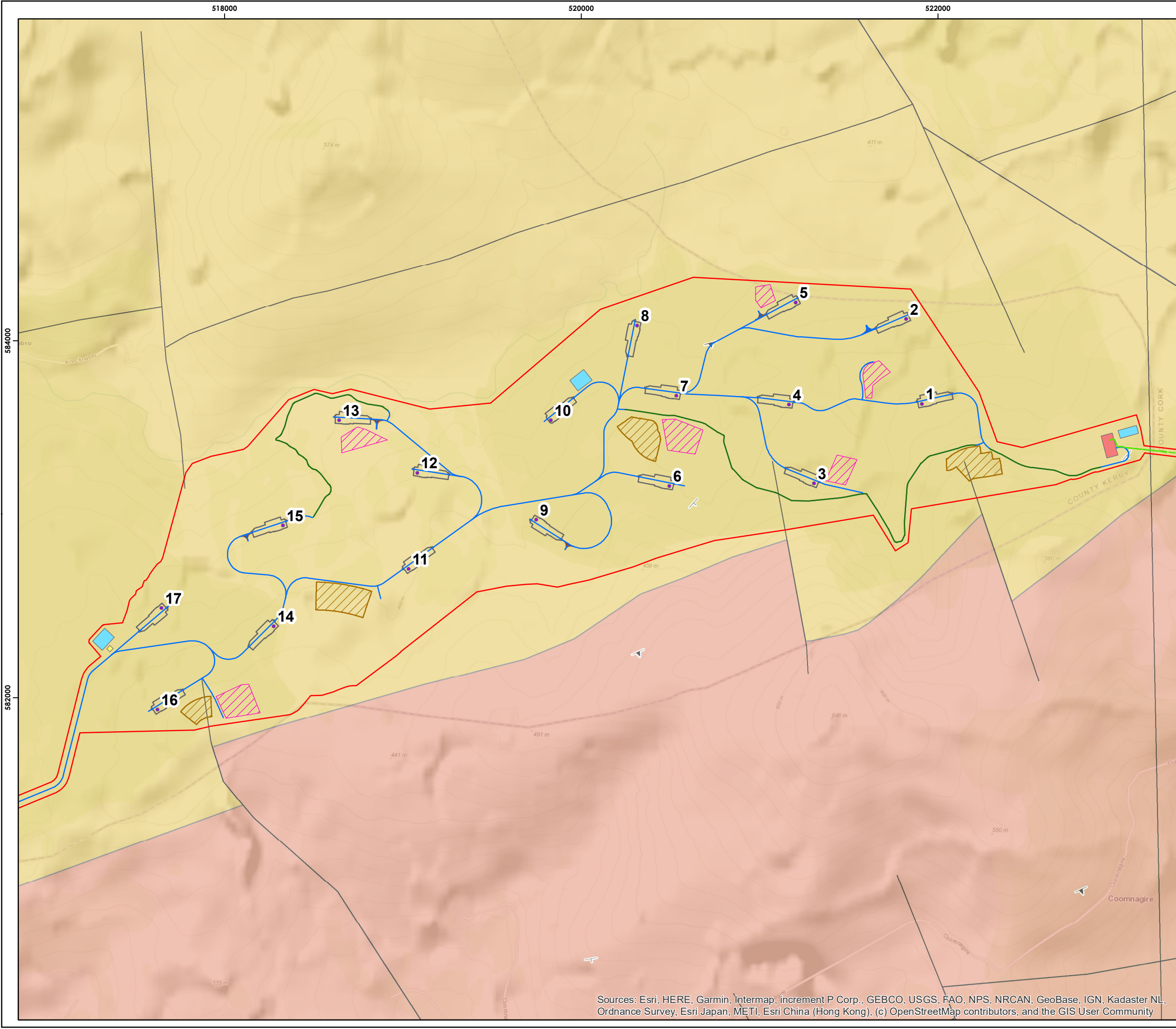
Figure10-3b Bedrock Geology
